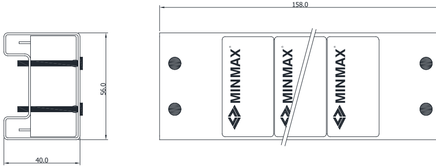
Unit: mm AMF-15 PCB Mounting 5 PCS per TUBE
