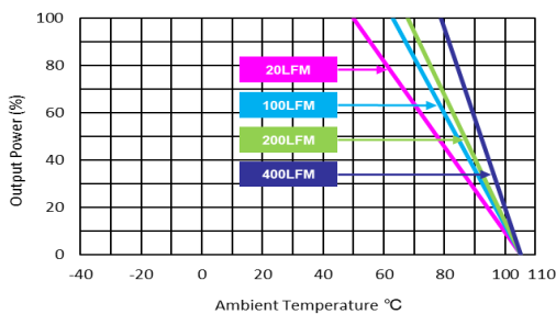
MJW25-12S05, MJW25-12S12, MJW25-12S15 MJW25-12D12, MJW25-12D15, MJW25-24D12 MJW25-24D15, MJW25-48D12, MJW25-48D15 Derating Curve without Heatsink
