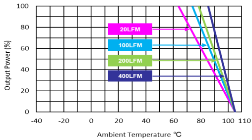
MJWI20-24S033 Derating Curve without Heatsink
