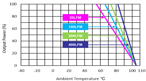
MJWI20-XXS24 Derating Curve without Heatsink
