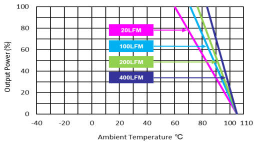
MJWI20-XXS05, MJWI20-XXS12, MJWI20-XXS15, MJWI20-XXD12, MJWI20-XXD15 Derating Curve without Heatsink
