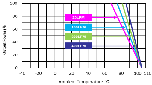
MJWI20-48S033 Derating Curve without Heatsink
