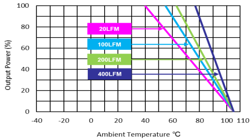
MKW40-XXDXX Derating Curve without Heatsink
