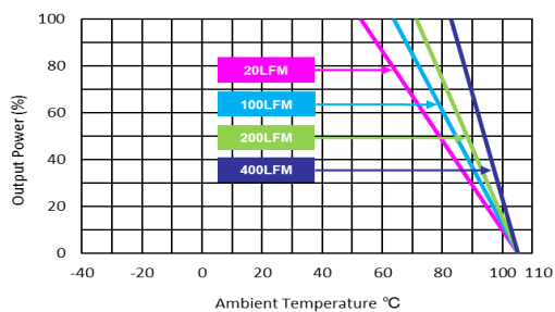
MKW150-24S12, MKW150-24S15, MKW150-48S12, MKW150-48S15 Derating Curve without Heatsink
